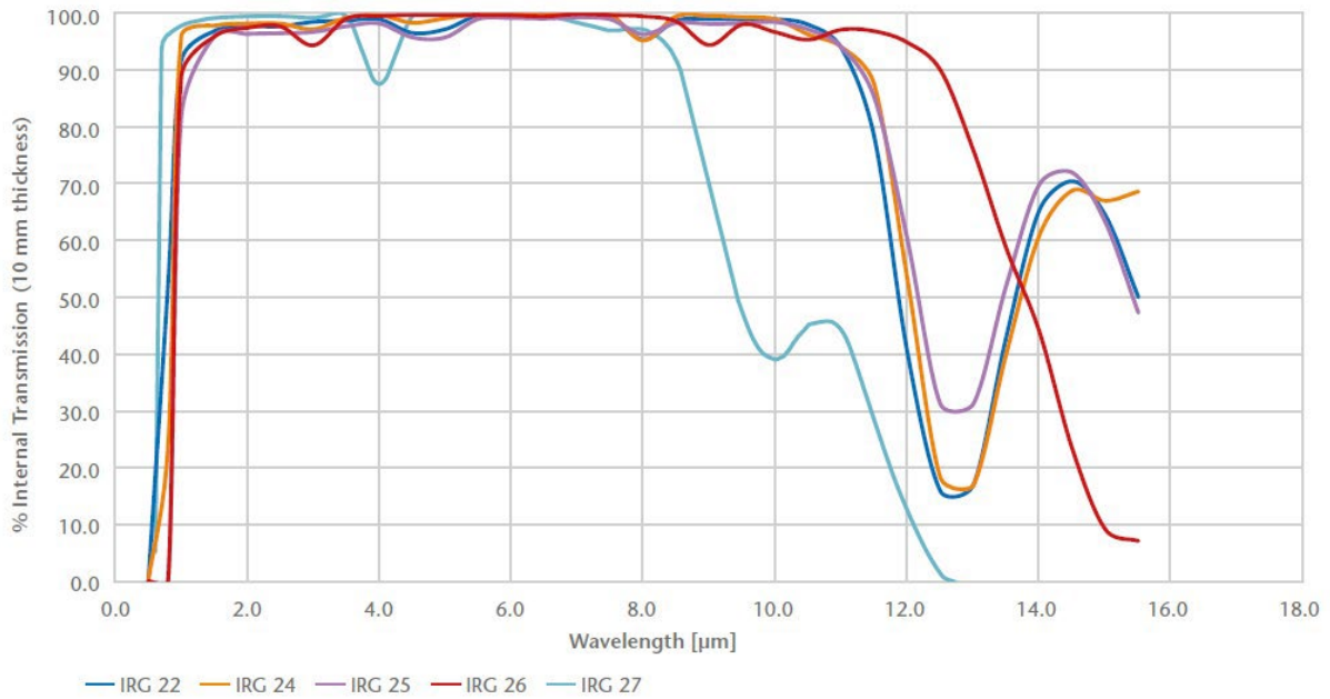
Internal Transmission of Infrared Glass IRG 22, IRG 24, IRG 25, IRG 26, IRG 27 with Thickness 10.0 mm (Typical Values)
